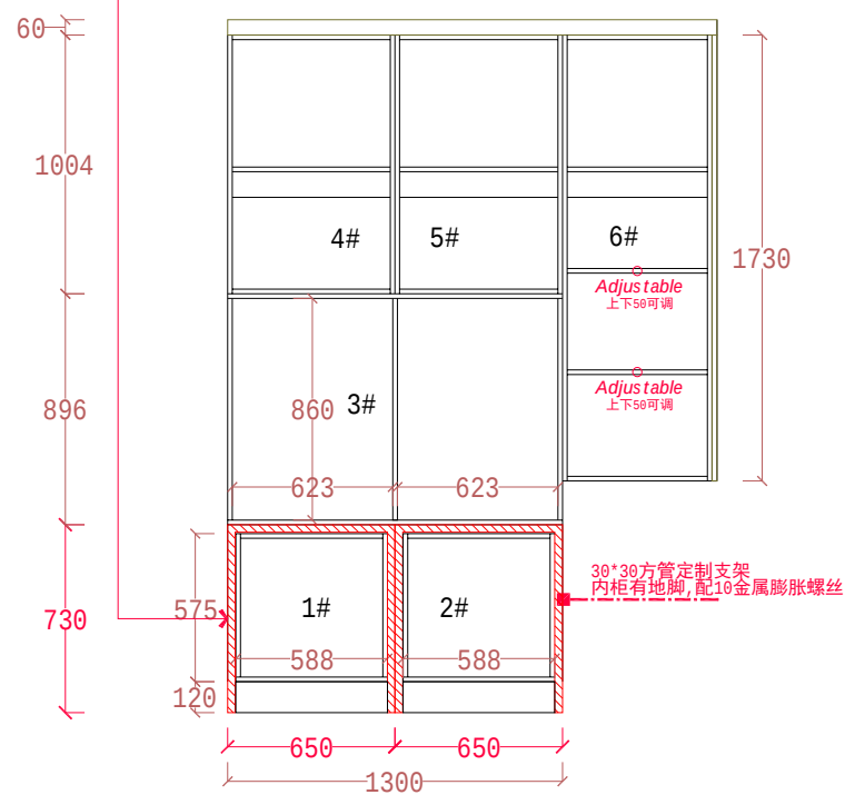
INNER VIEW A
