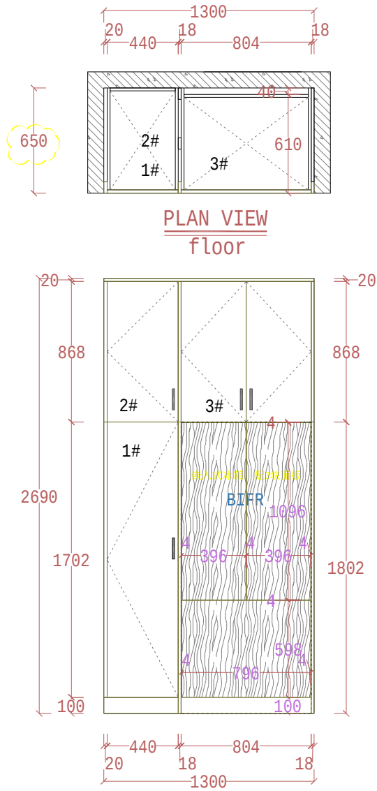
ELEVATION D
