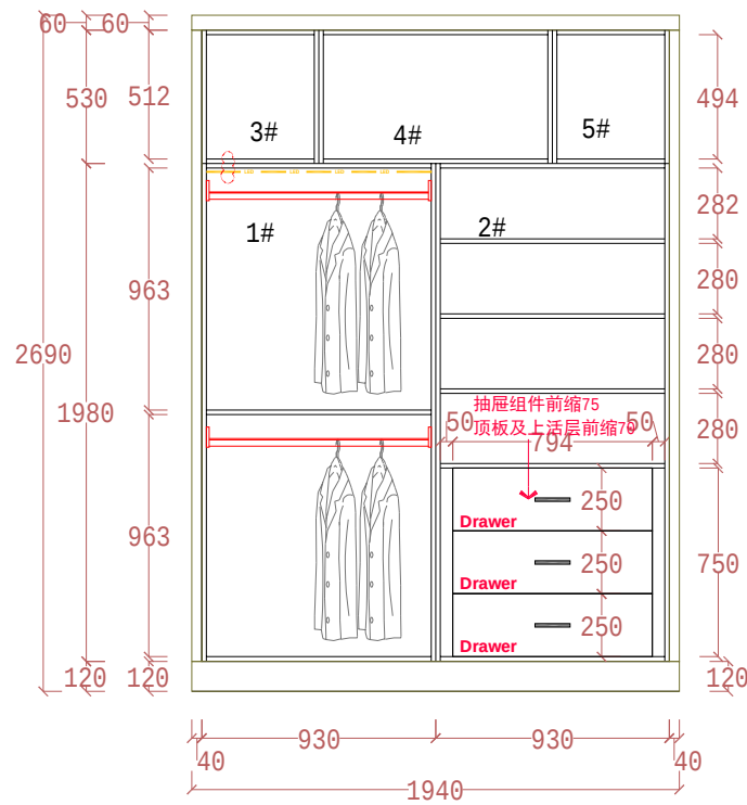
INNER VIEW
