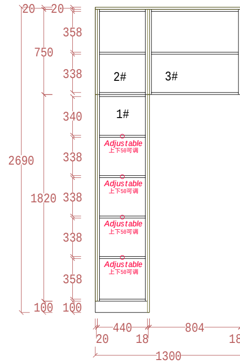
INNER VIEW D
