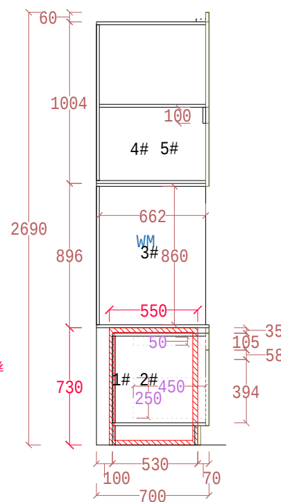
SECTION VIEW
