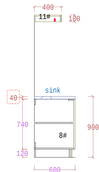
SECTION VIEW
