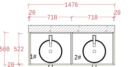
PLAN VIEW floor
