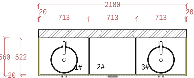
PLAN VIEW floor
